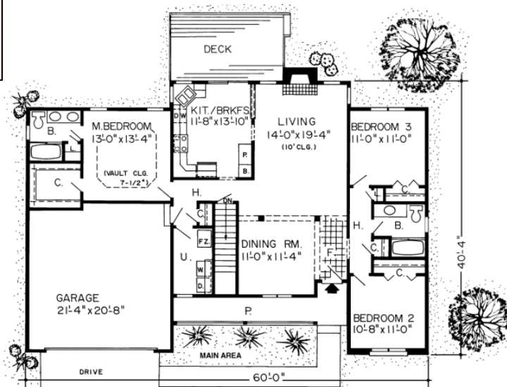
Alternate Crawl/Slab Plan
